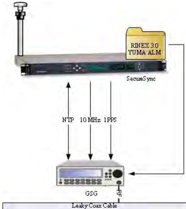
Fig. 1 Intelligent Repeater System – Single Zone
